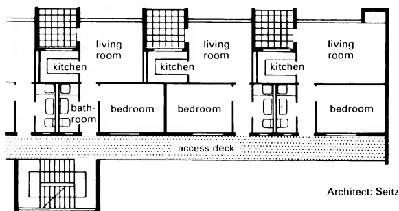
⑤ Stairway installed in front of the access deck: kitchens are lit and ventilated via an inset balcony
